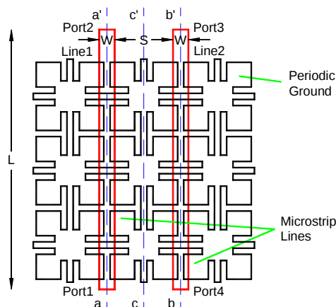
Fig. 1. Parallel microstrip lines on the top of a dielectric substrate, while a periodic structure is serving as the ground plane.
