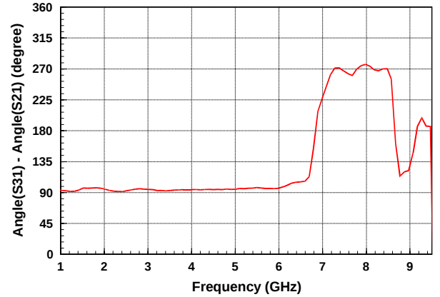
Fig. 6. Difference of phase angle between S_{31} and S_{21} .
