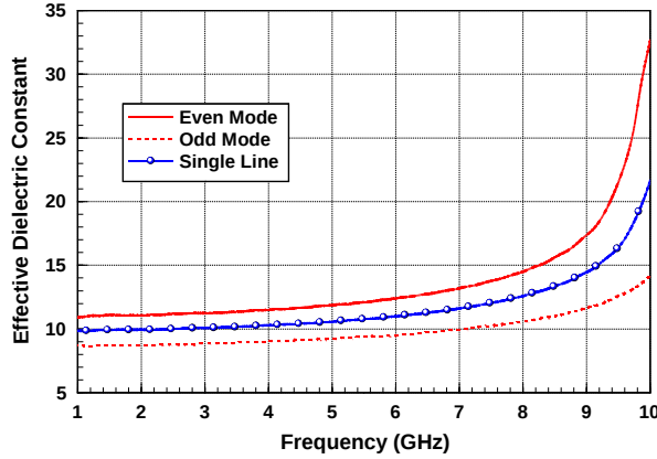
Fig. 4. Simulated effective dielectric constant.
