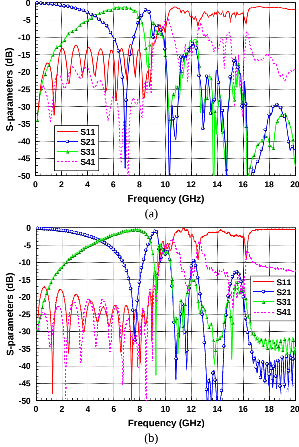
Fig. 2. (a) Measured and (b) simulated S-parameters.
