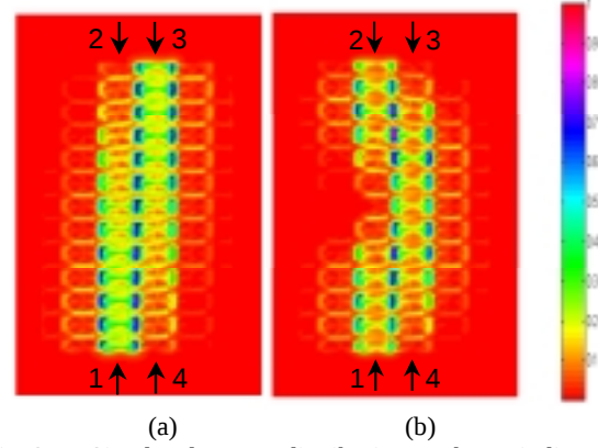
Fig. 3. Simulated current distribution on the periodic ground plane at (a) 7 GHz and (b) 9 GHz.
